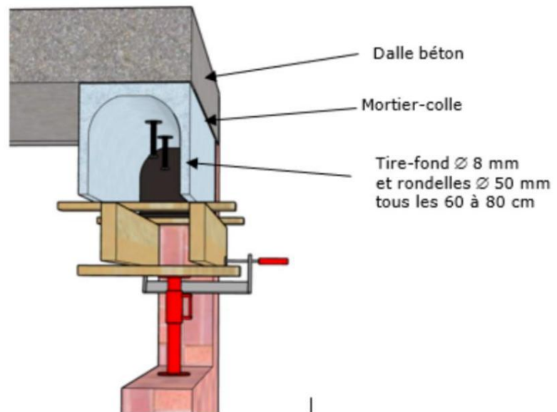
Figure 31 - Installation under slab with lag screws placed every 60 to 80 cm
