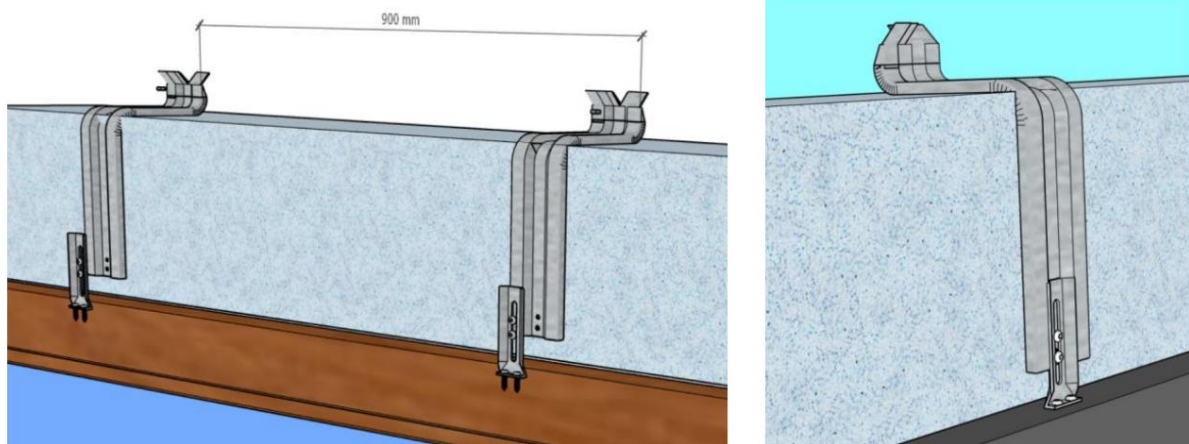
Figure 40 - RT2830 reinforcement allowing the joinery to hold to the lintel
