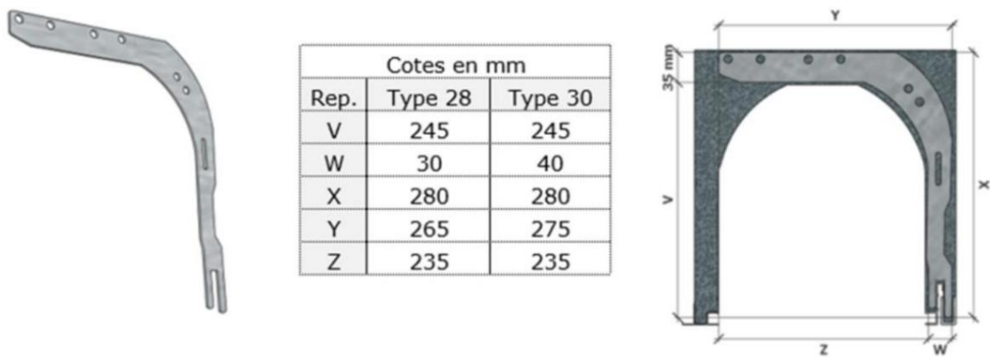
Figure 24 - Galvanized steel reinforcement for reinforced boxes
