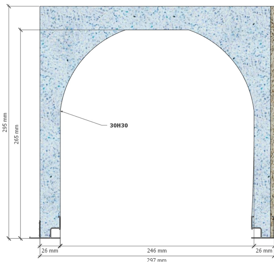
Box shown: C-30H30 8-8H F
